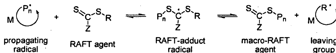
Scheme 1: Proposed mechanism for RAFT polymerisation, where M represents monomer, P_n represents polymerised monomer, and Z and R are as defined below.
