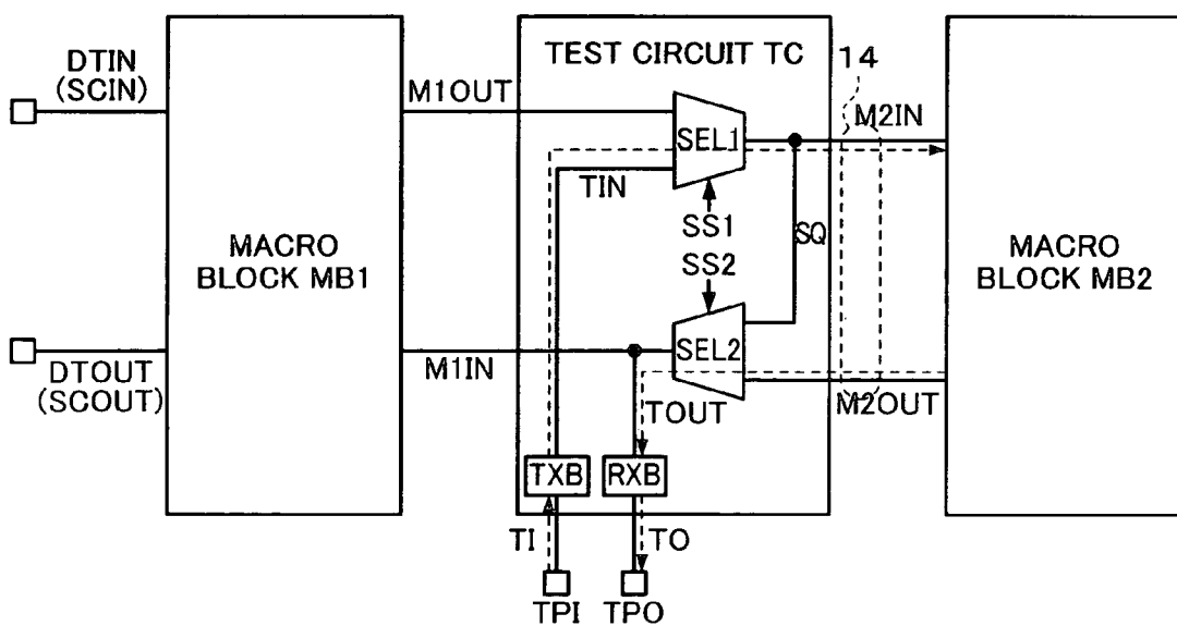
FIG. 7B SECOND TEST MODE
