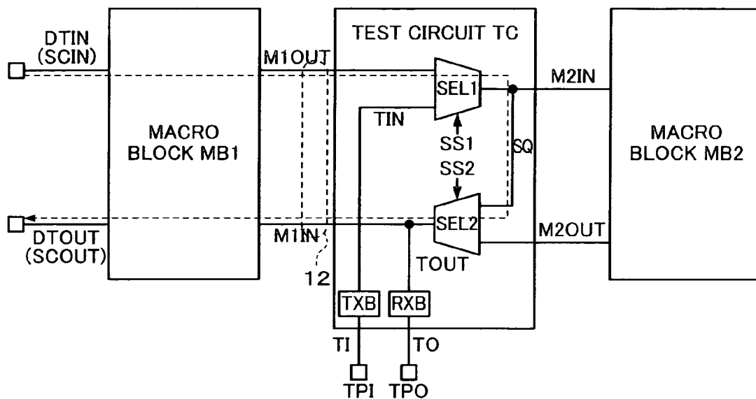
FIG. 7A FIRST TEST MODE
