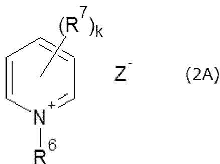
[Chemical Formula 8]
