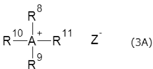
[Chemical Formula 8]
