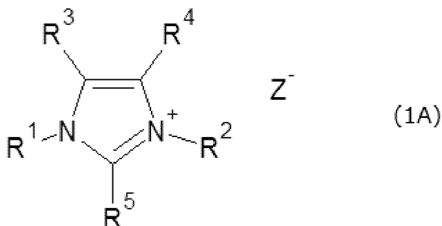
[Chemical Formula 7]
