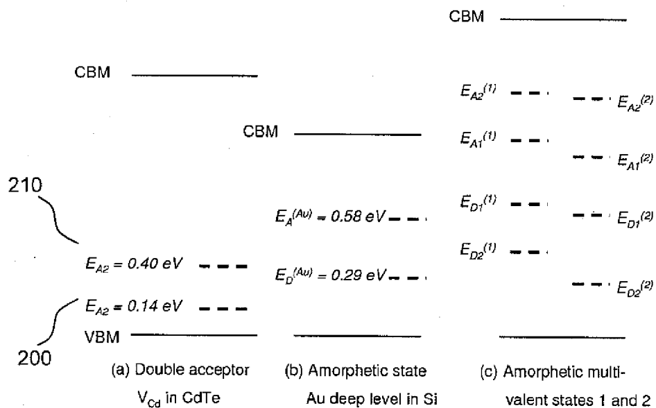
Figure 2 (Prior Art)
