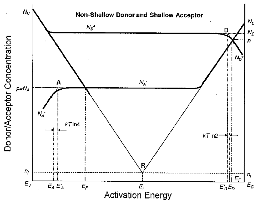
Figure 1 (Prior Art)
