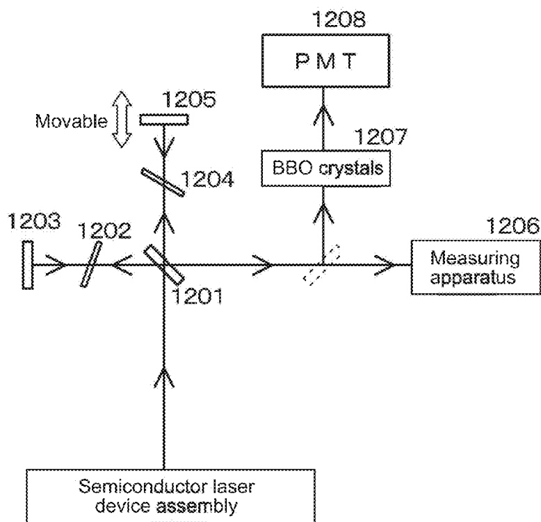
FIG. 32 PRIOR ART
