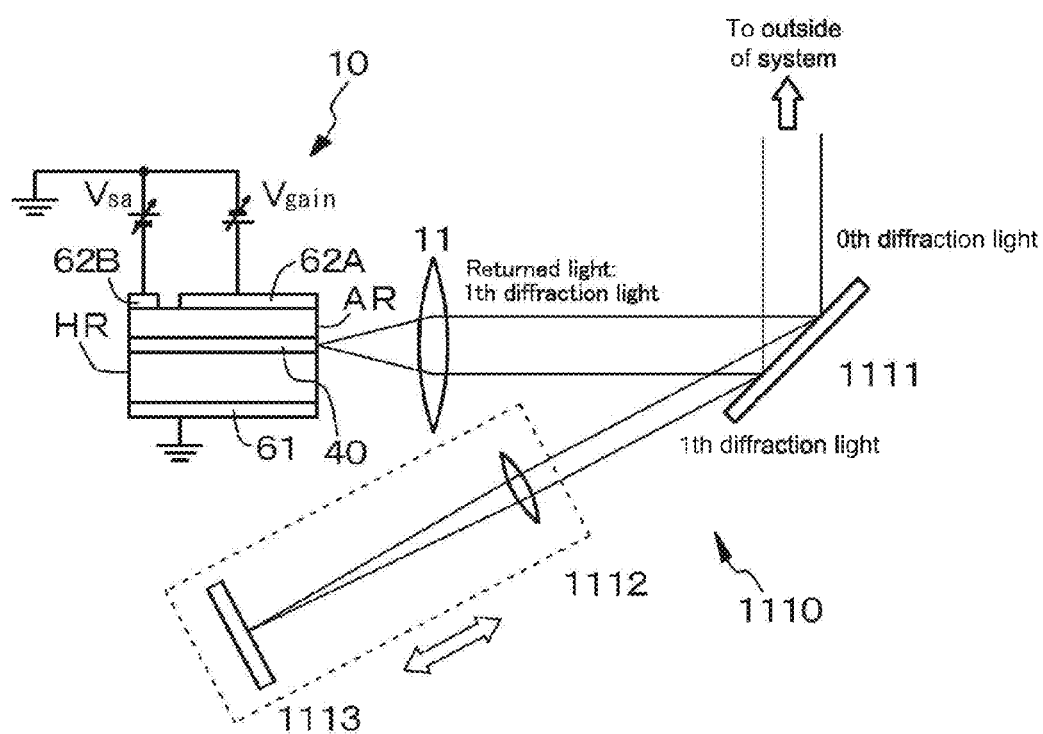
FIG.29 PRIOR ART
