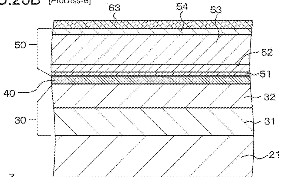
FIG.26B [Process-B]
