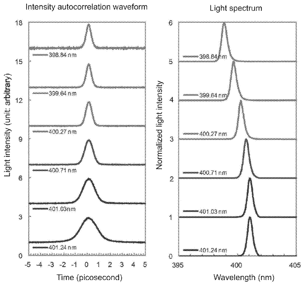
FIG.35 PRIOR ART
