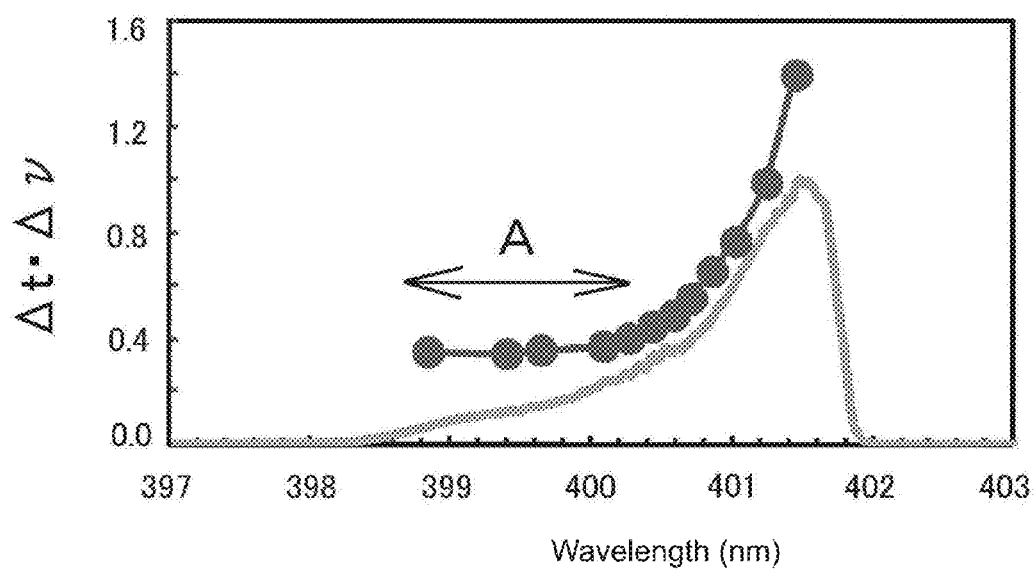
FIG.36 PRIOR ART
