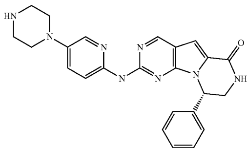
Compound 23
