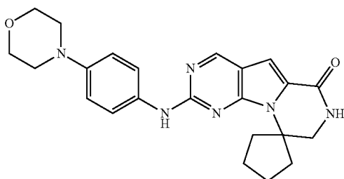
Compound 34 10
