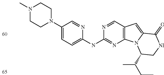
Compound 16
