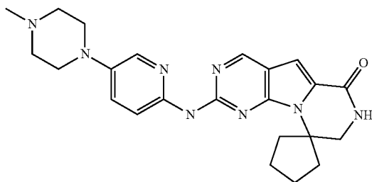
Compound 29
