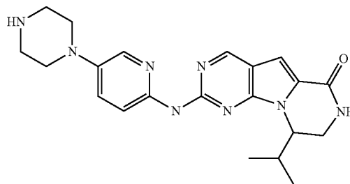
Compound 8
