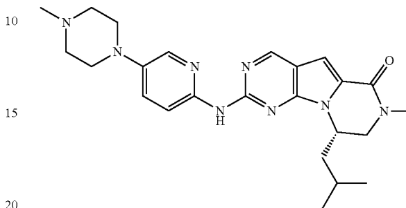
Compound 14
