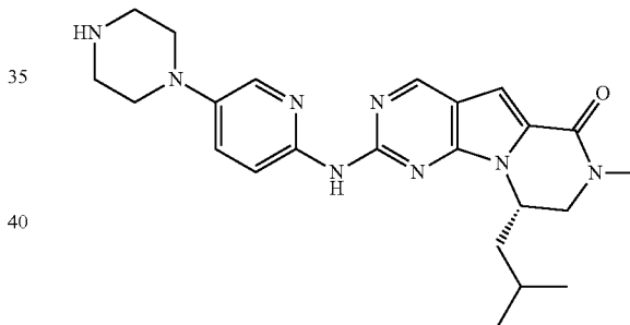
Compound 15
