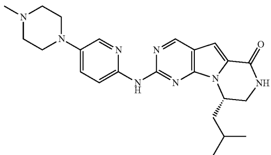
Compound 12
