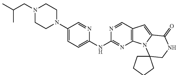
Compound 36
