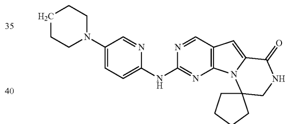
Compound 38
