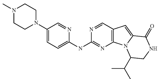
Compound 7
