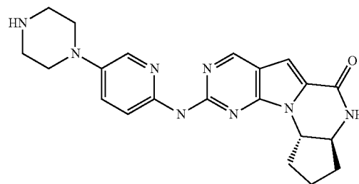
Compound 49
