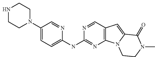
Compound 5
