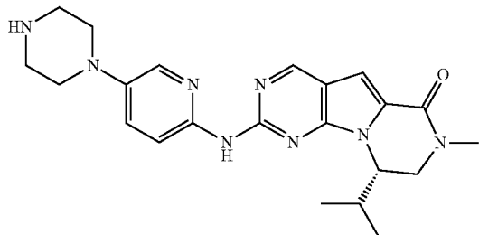
Compound 11
