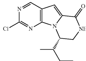
tert-butyl N-[(2S)-2-[(5-bromo-2-chloro-pyrimidin-4-yl)amino]-3-methyl-pentyl]carbamate
