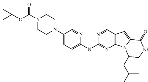
Compound 50
