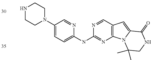
Compound 26
