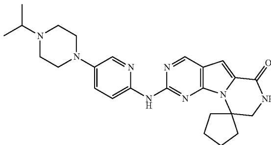
Compound 35
