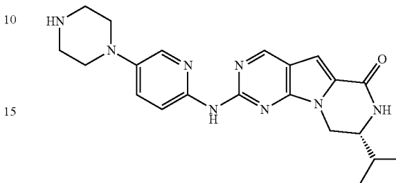
Compound 25
