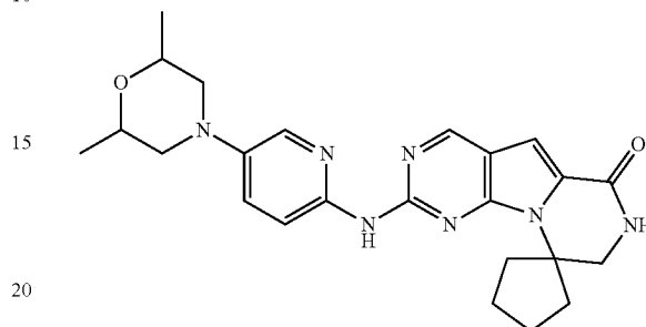
Compound 37
