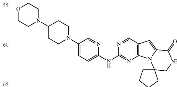
Compound 39
