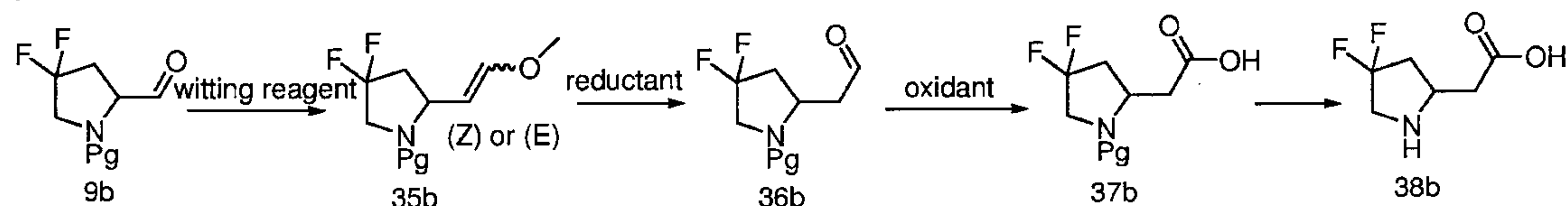
Scheme 7
