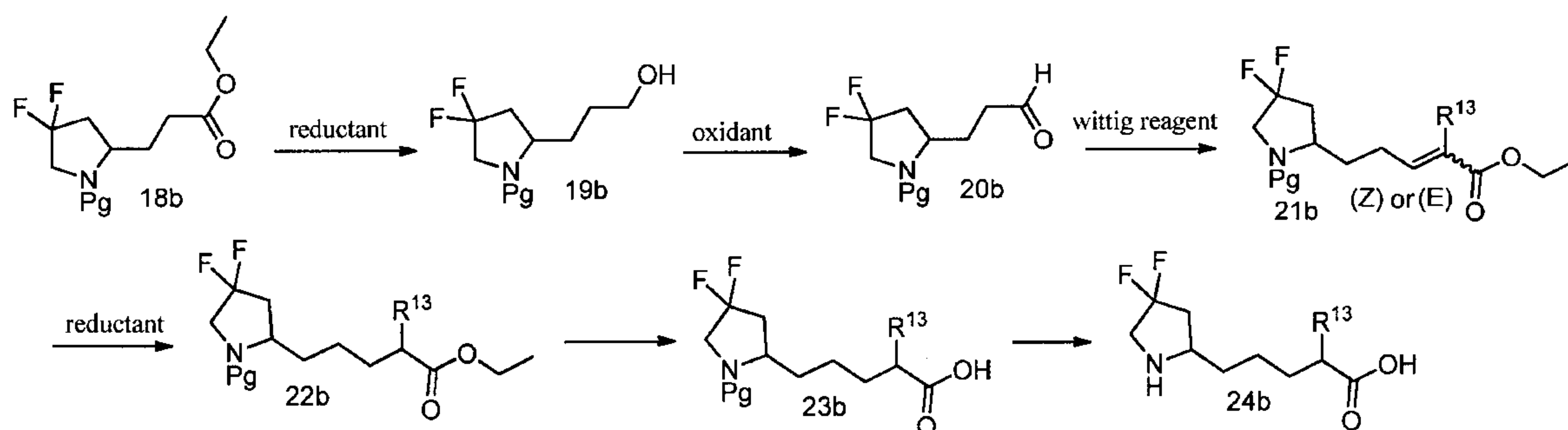
Scheme 5
