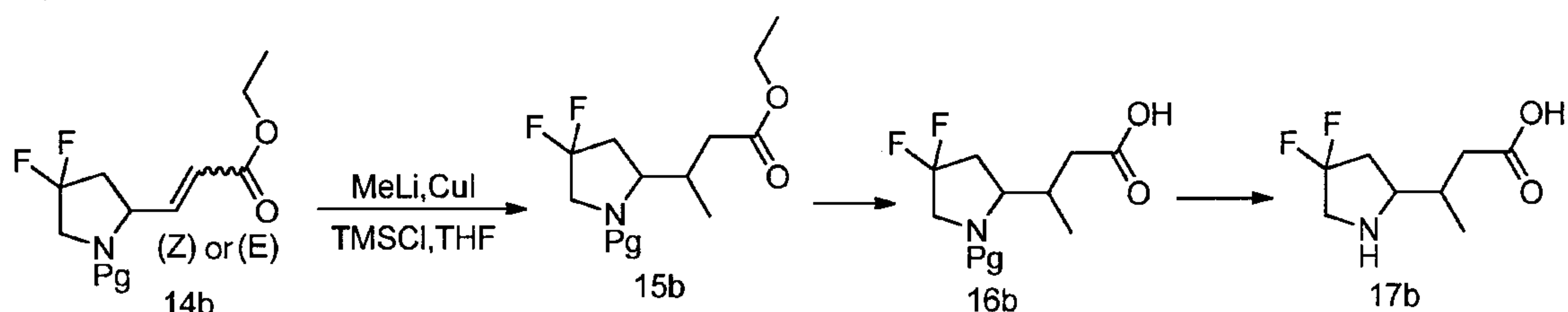
Scheme 4
