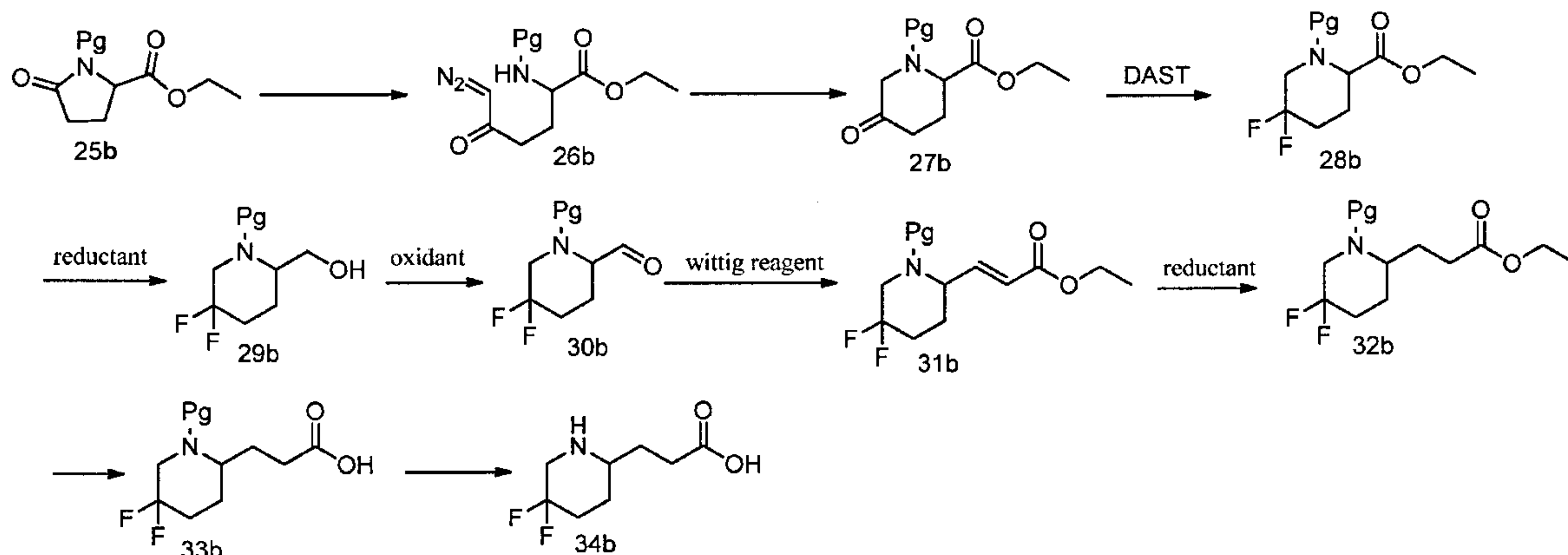
Scheme 6
