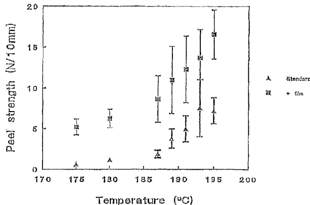
COMPACTED PP - 10:1 6060 Effect of interleaved film
