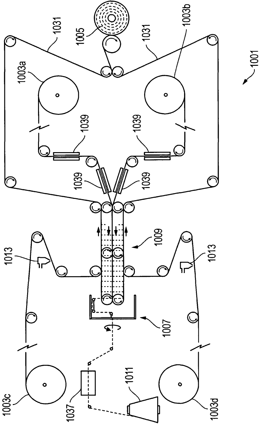
FIG. 6 (Prior Art)
