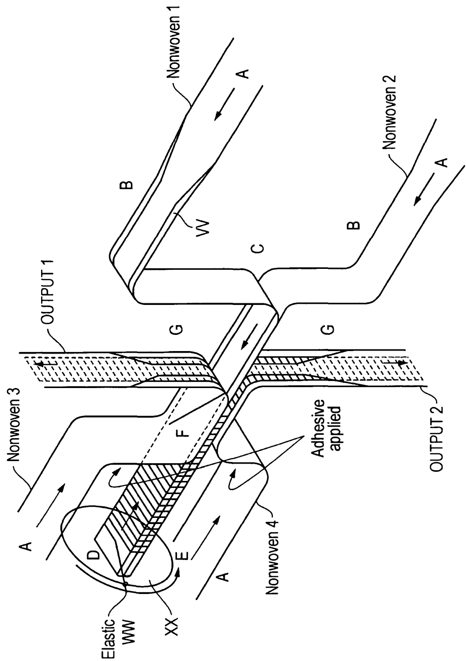
FIG. 9 (PRIOR ART)
