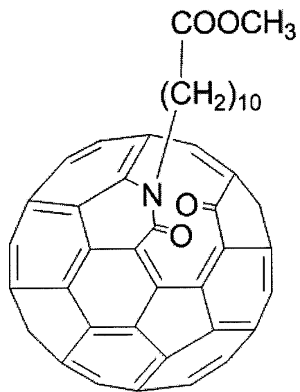
KetoEster1
