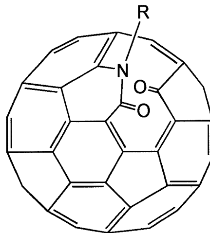
Molecule 1
