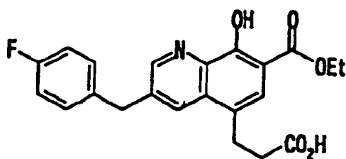
Compound [A]
