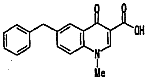
Compound [G]
