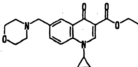
Compound [H]
