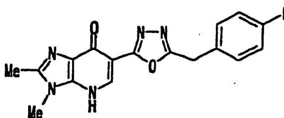
Compound [B]
