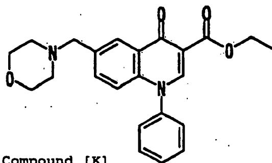
Compound [K]
