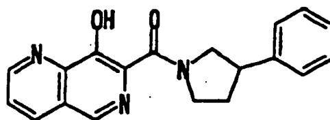
Compound [D]
