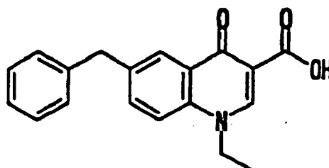
Compound [E]
