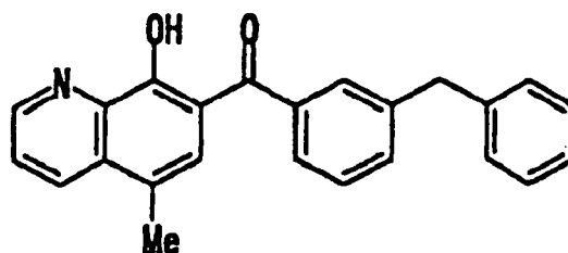
Compound [C]
