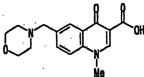
Compound [J]
