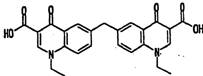
Compound [F]
