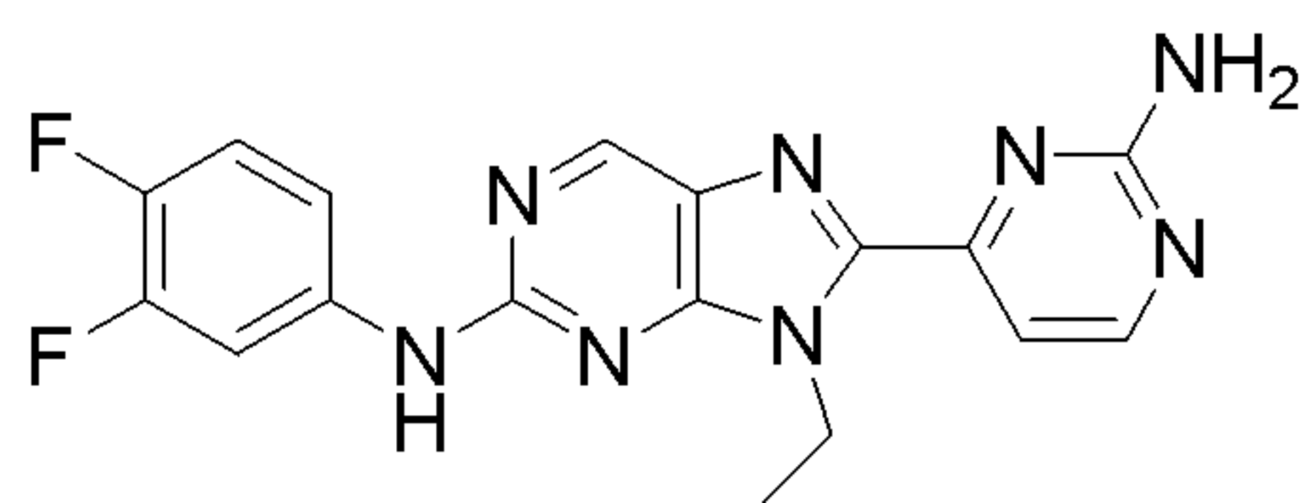
[00213] 8-(2-Aminopyrimidin-4-yl)-N-(3,4-difluorophenyl)-9-ethyl-9H-purin-2-amine
