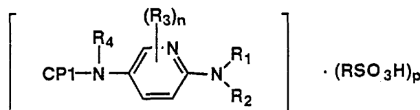
Formula 2
