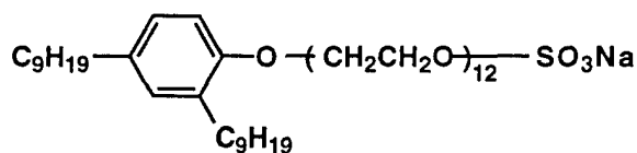
Compound J
