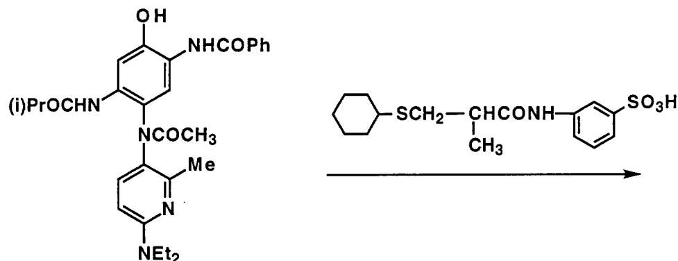
Exemplified compound 8
