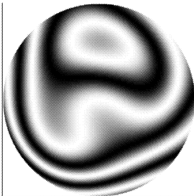
1.064um Interferogram showing basic WFE generated by DM-1 \sim 500
