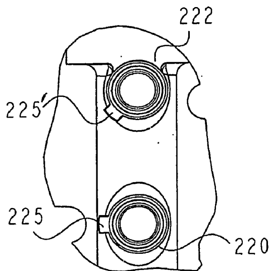
DETAIL B SCALE 2.000
