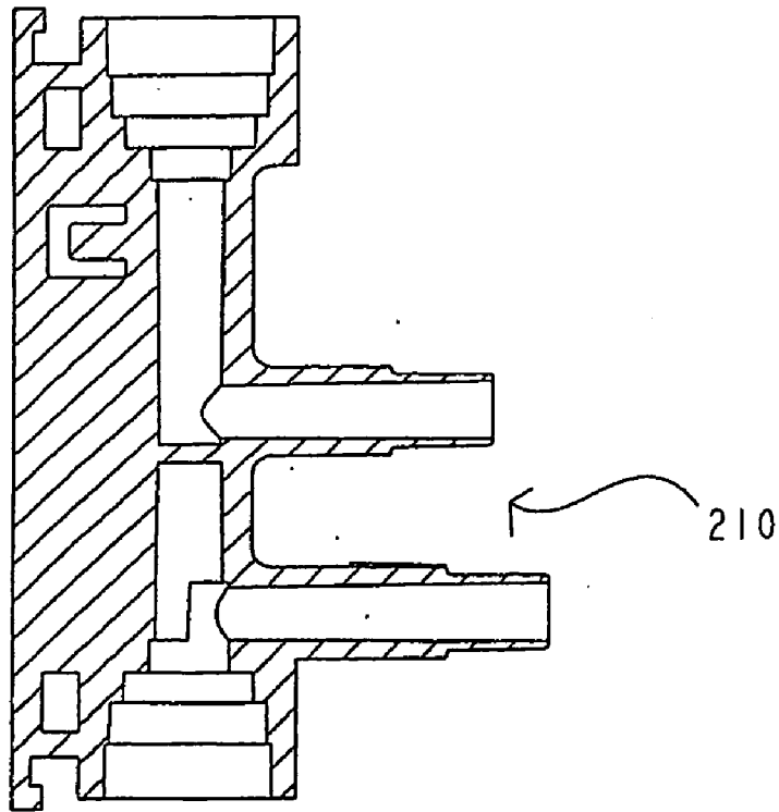
SECTION B-B
