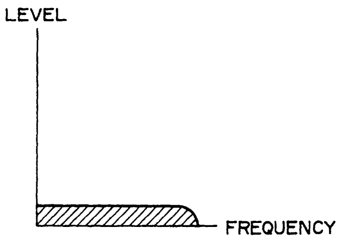
ANTI-DUPLICATION CONTROL SIGNAL SPECTRUM AFTER SPECTRAL SPREAD
