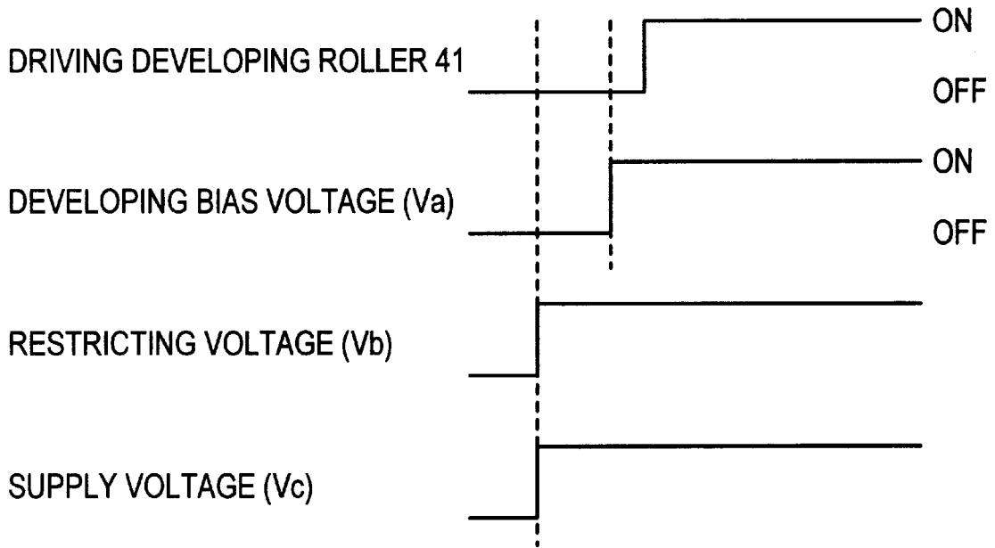
FIG. 4A START OF IMAGE FORMING PROCESSING
