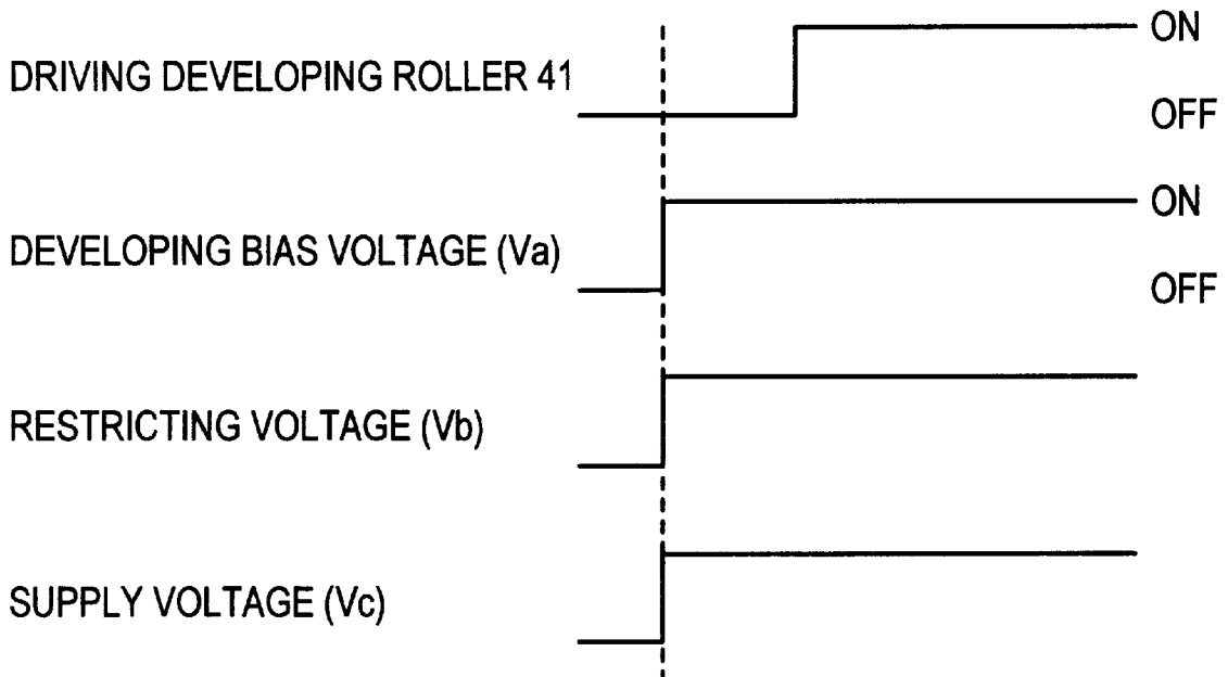
FIG. 2A START OF IMAGE FORMING PROCESSING
