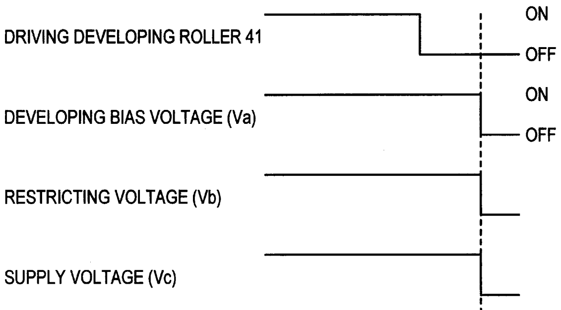
FIG. 2B END OF IMAGE FORMING PROCESSING
