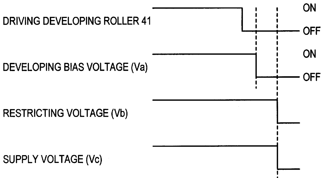
FIG. 4B END OF IMAGE FORMING PROCESSING
