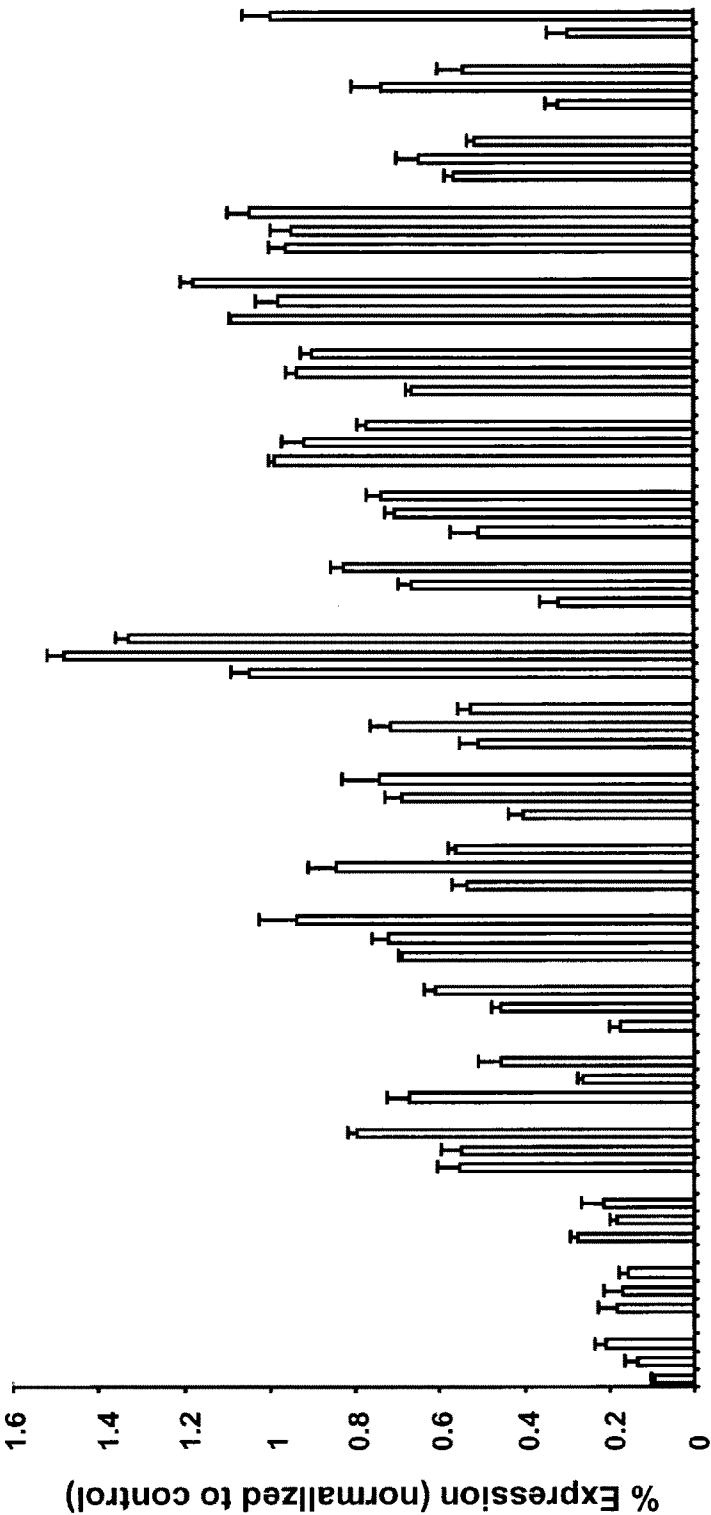
siRNA 100 nM
