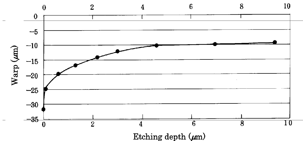
Relationship between wet etching depth and warp
