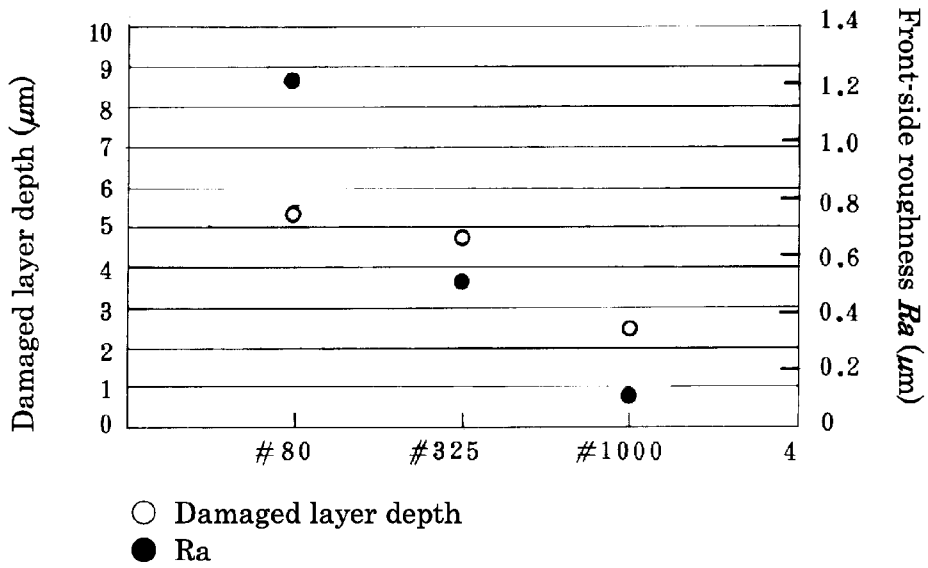
Post-grinding relationship between damaged layer and surface roughness
