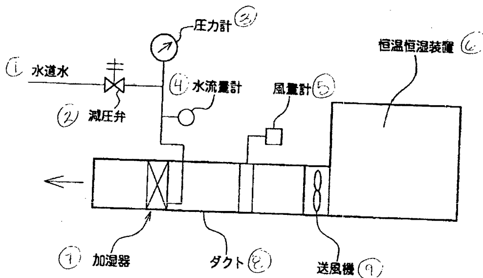
Fig. 12 Humidification Performance Measuring System
