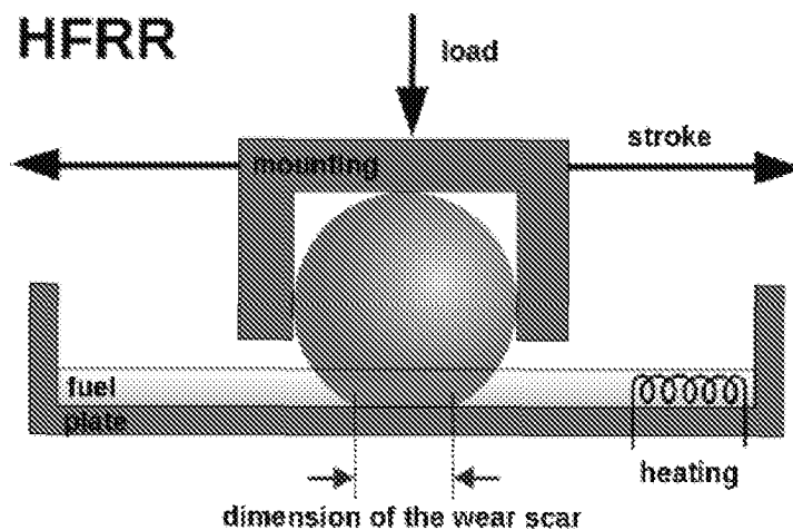
Figure 6: couplings of the HFRR test
