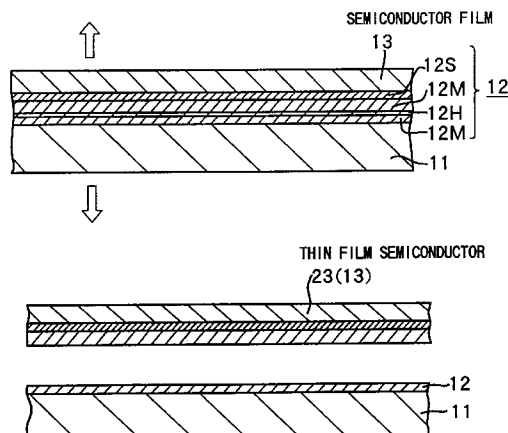
PROCESS DIAGRAM (SECOND)
