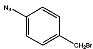
Compound 10
