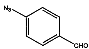
Compound 7
