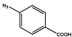
Compound 6
