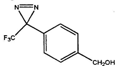
Compound 4
