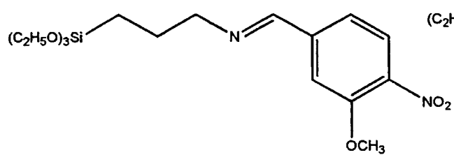
Compound 18
