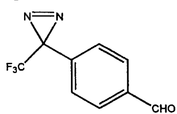
Compound 2
