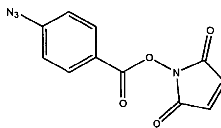
Compound 8
