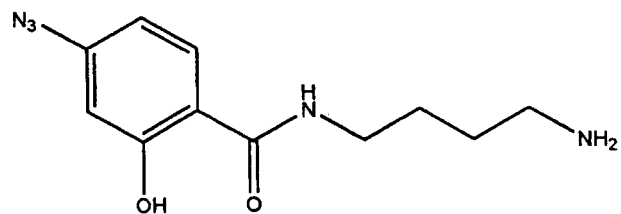
Compound 26
