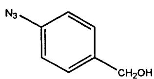
Compound 9
