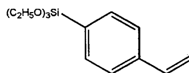
Compound 16
