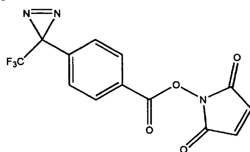
Compound 3
