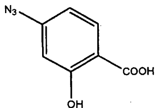
Compound 27
