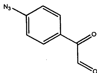
Compound 25
