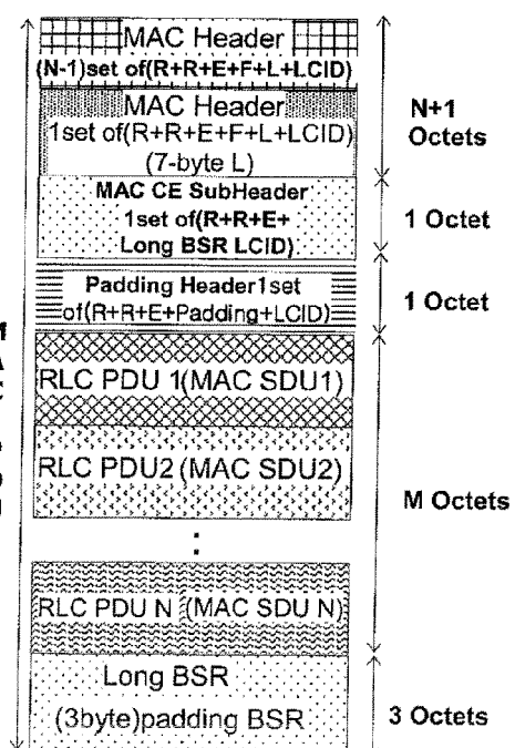
(c) case 3, 7-bit L field for the last MAC SDU
