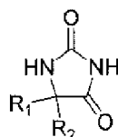
IIb R_1 = \text{CH}_3 , R_2 = -\text{CH}_2\text{COOC}_2\text{H}_5
