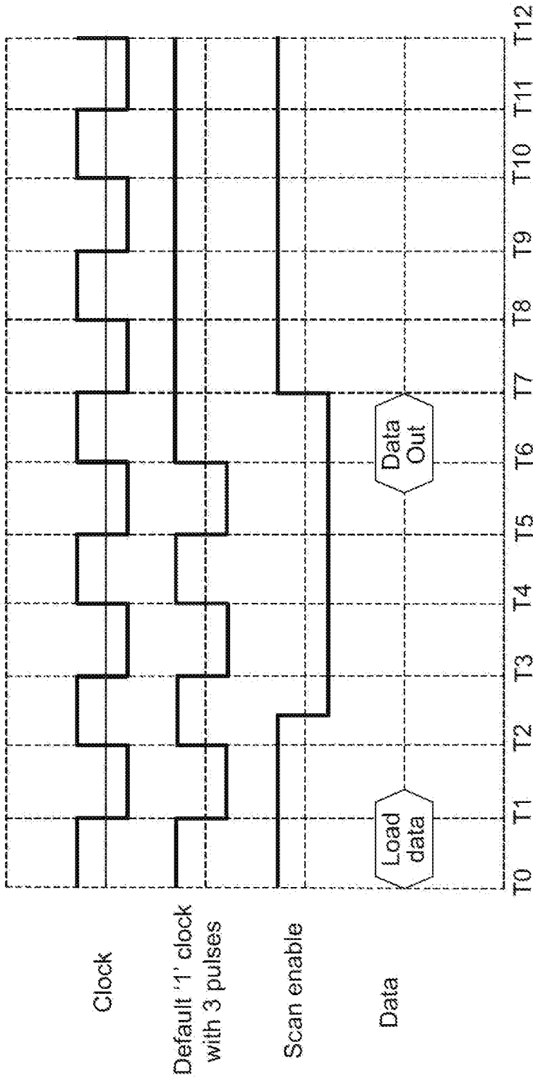
Testing of logic circuitry 580
