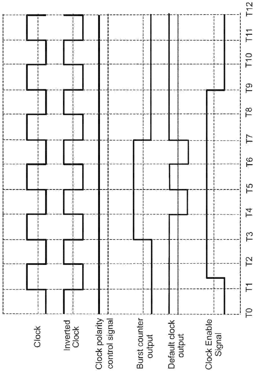
Generation of default clock '1' with two pulses
