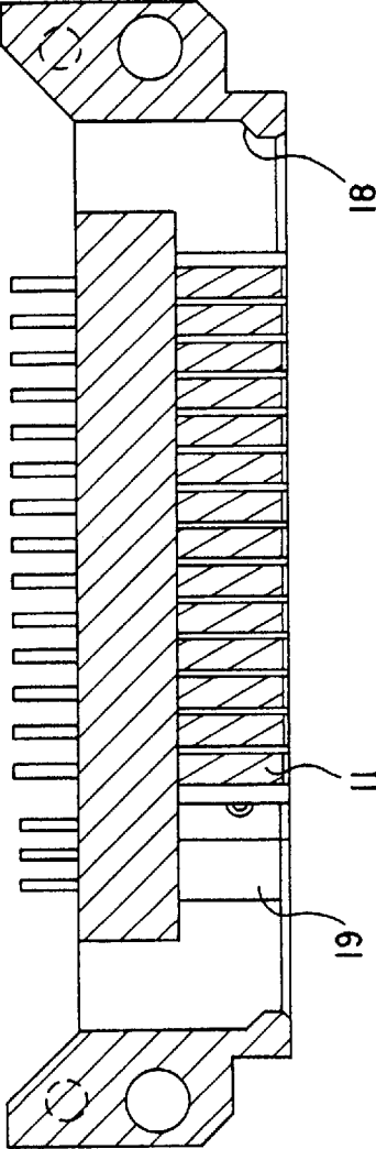
FIG.3C
