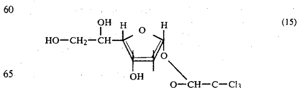
\beta -(di-trichloroethylidene)-d-gluco-furanose:
