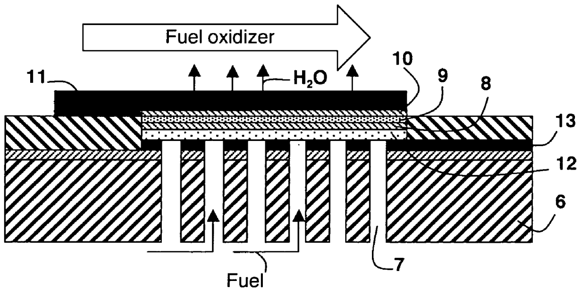
Fig.2 (Prior art)
