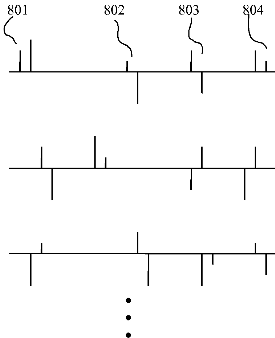
FIG.8 Proposed Dual-Pulse Excitation Codebook
