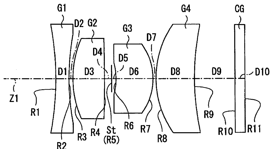
ARRANGEMENT 1 (EXAMPLE 1)
