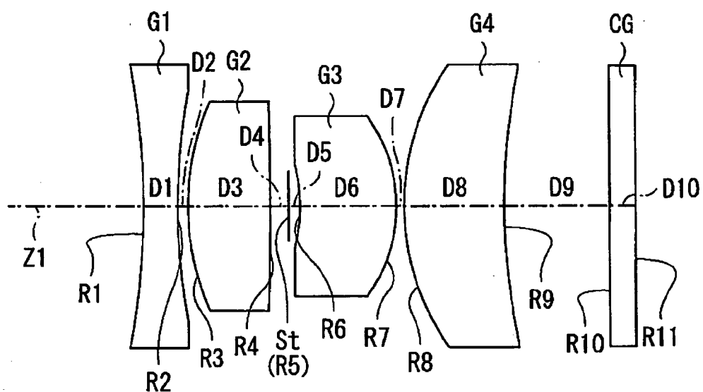
ARRANGEMENT 1 (EXAMPLE 1)
