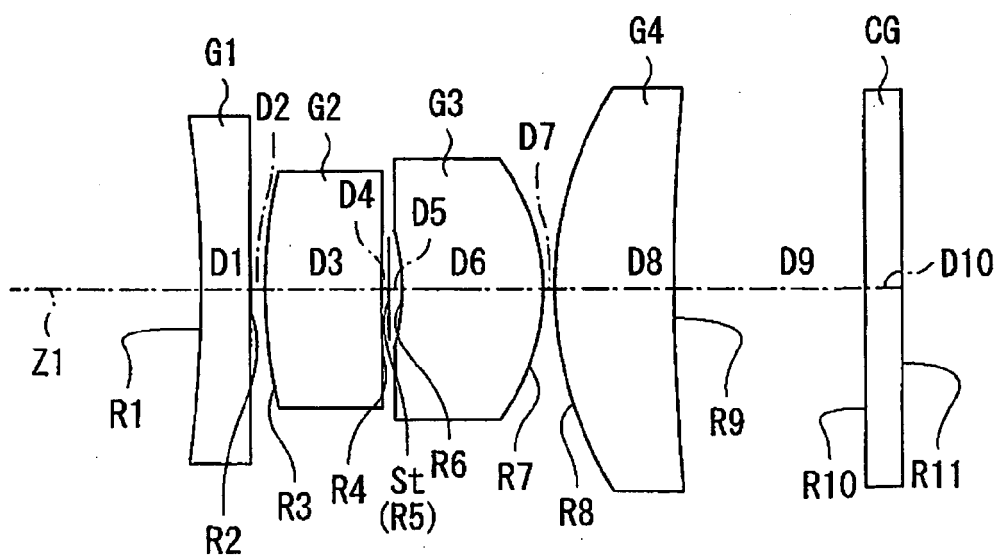
ARRANGEMENT 2 (EXAMPLE 5)
