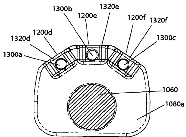
FIG. 1ee (Section A-A of Fig. 1aa)
