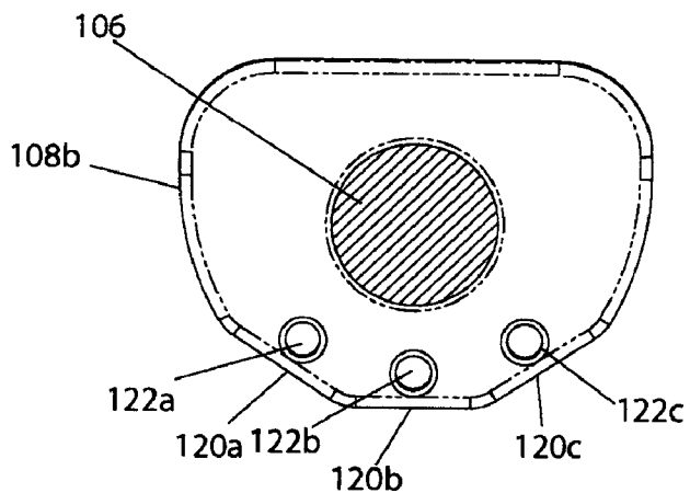
FIG. 1f (Section B-B of Fig. 1a)
