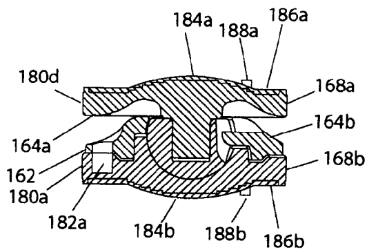
FIG. 1h (Section C-C on Fig. 1i)
