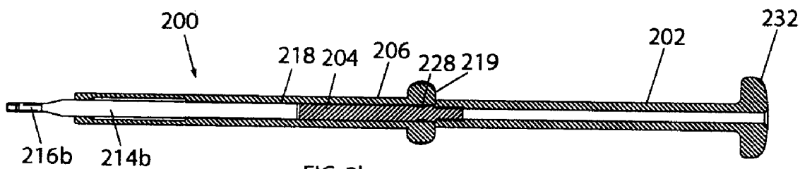
FIG. 2k (Section A-A of Fig. 2b)
