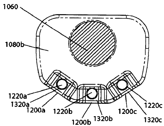
FIG. 1ff (Section B-B of Fig. 1aa)
