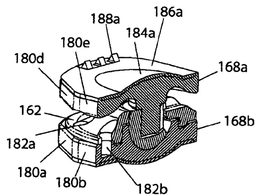
FIG. 1j (Perspective of Fig. 1h)
