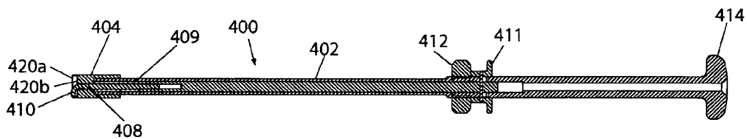
FIG. 4c (Section A-A of Fig. 4b)
