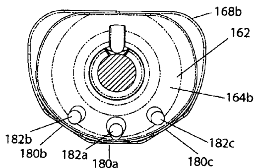
FIG. 1l (Section B-B on Fig. 1g)
