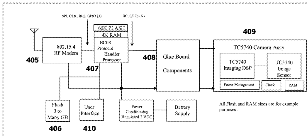
Camera End Node (40) Block Diagram
