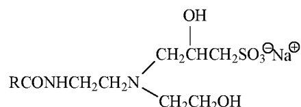
AMPHOTERIC SULFONATE
