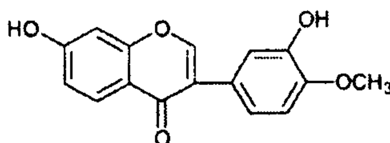
Calycosin
