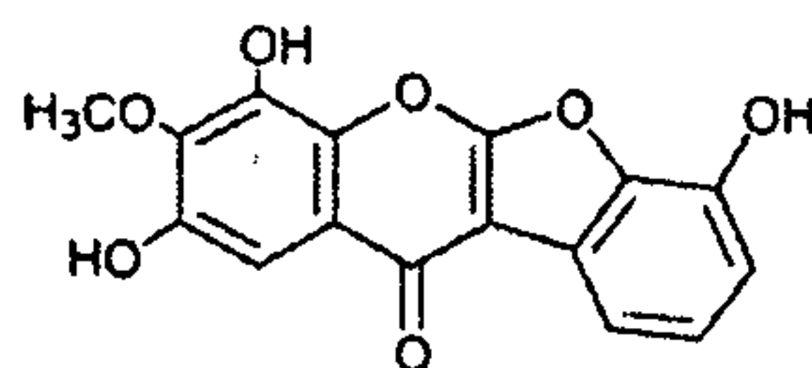
Tetracyclic isoflavone
