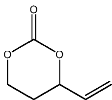
(Formula IV-6),
