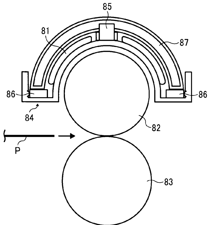
FIG. 18 RELATED ART
