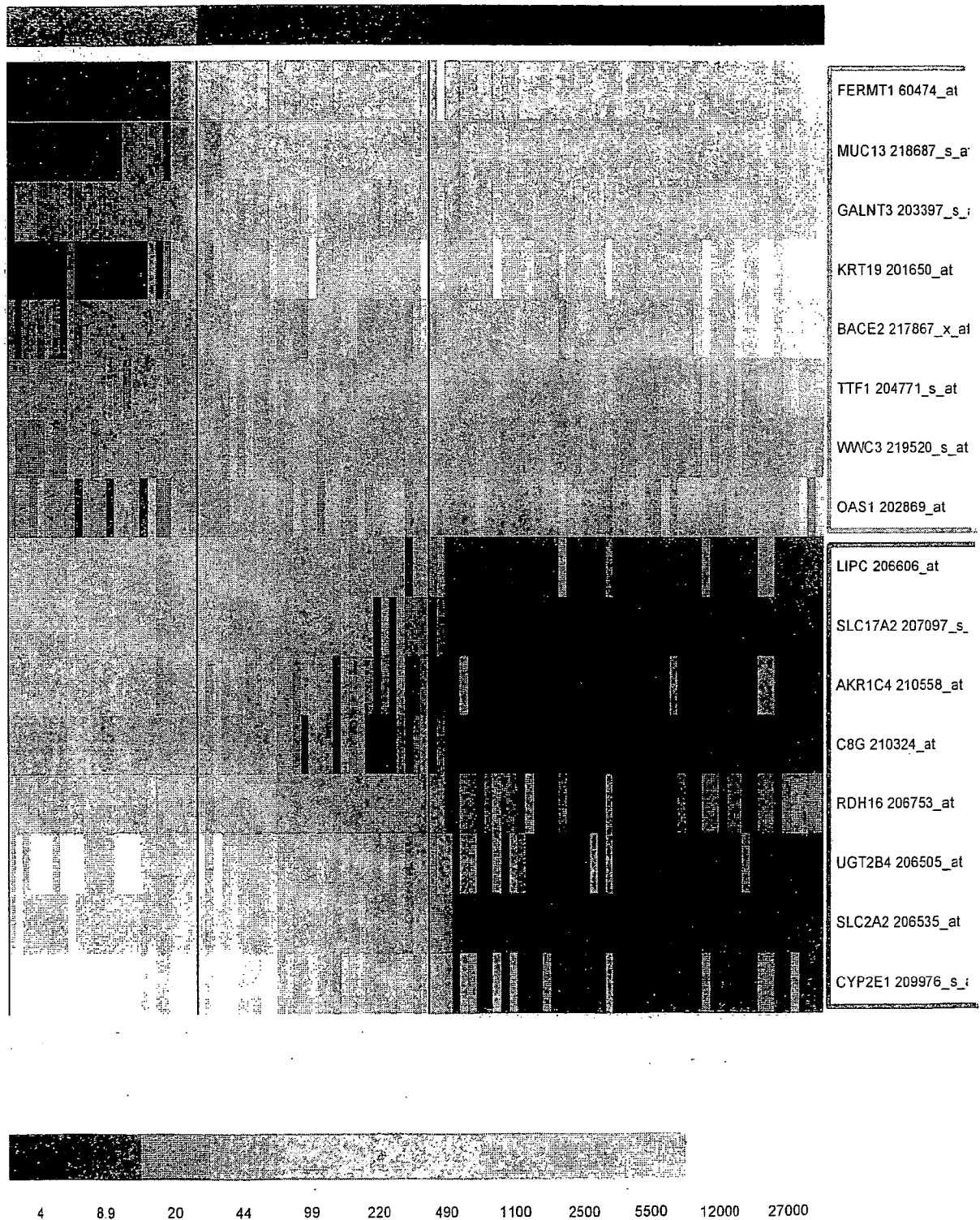
Fig. 16: Identification of RNA samples with high (grey), medium (dark grey) and low (black) liver contamination based on expression of genes predominantly expressed in colorectal cancer (upper box) and normal liver (lower box). The color scale reflects the absolute element signal intensity after normalization.
