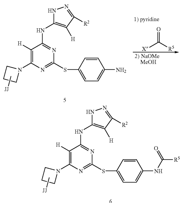
Scheme II
