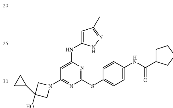
N-(4-((4-(3-methyl-1H-pyrazol-5-ylamino)-6-(3-cyclopropyl-3-hydroxyazetidin-1-yl)pyrimidin-2-yl)sulfanyl)phenyl)cyclopentanecarboxamide (I-9)
