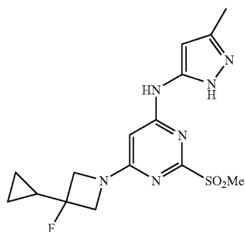
6-(3-cyclopropyl-3-fluoroazetidin-1-yl)-N-(3-methyl-1H-pyrazol-5-yl)-2-(methylsulfonyl)pyrimidin-4-amine
