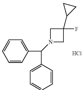
1-Benzhydryl-3-cyclopropyl-3-fluoroazetidine Hydrochloride
