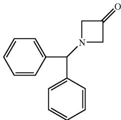
N-Benzhydrylazetidin-3-one
