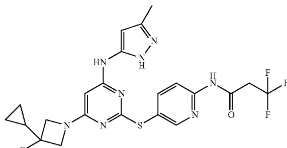
N-(5-(4-(3-methyl-1H-pyrazol-5-ylamino)-6-(3-cyclopropyl-3-fluoroazetidin-1-yl)pyrimidin-2-ylthio)pyridin-2-yl)-3,3,3-trifluoropropanamide (I-21)
