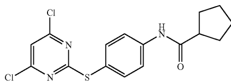
N-(4-(4,6-dichloropyrimidin-2-ylthio)phenyl)cyclopentanecarboxamide
