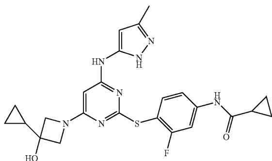
N-4-((4-(3-methyl-1H-pyrazol-5-ylamino)-6-(3-cyclopropyl-3-hydroxyazetidin-1-yl)pyrimidin-2-yl)thio)-3-fluorophenyl)cyclopropanecarboxamide (I-11)
