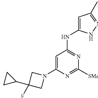
6-(3-cyclopropyl-3-fluoroazetidin-1-yl)-N-(3-methyl-1H-pyrazol-5-yl)-2-(methylthio)pyrimidin-4-amine
