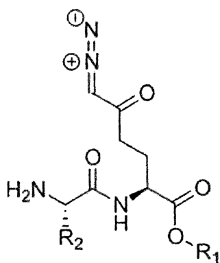
25 ( R_1 = \text{Et}, R_2 = \text{iBu} ) 9 ( R_1 = \text{iPr}, R_2 = \text{iBu} ) 34 ( R_1 = \text{Et}, R_2 = -\text{CH}_2\text{-3-indolyl} ) 38 ( R_1 = \text{iPr}, R_2 = -\text{CH}_2\text{-3-indolyl} )
