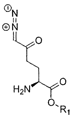
20 ( R_1 = \text{Et} ) 3 ( R_1 = \text{iPr} )
