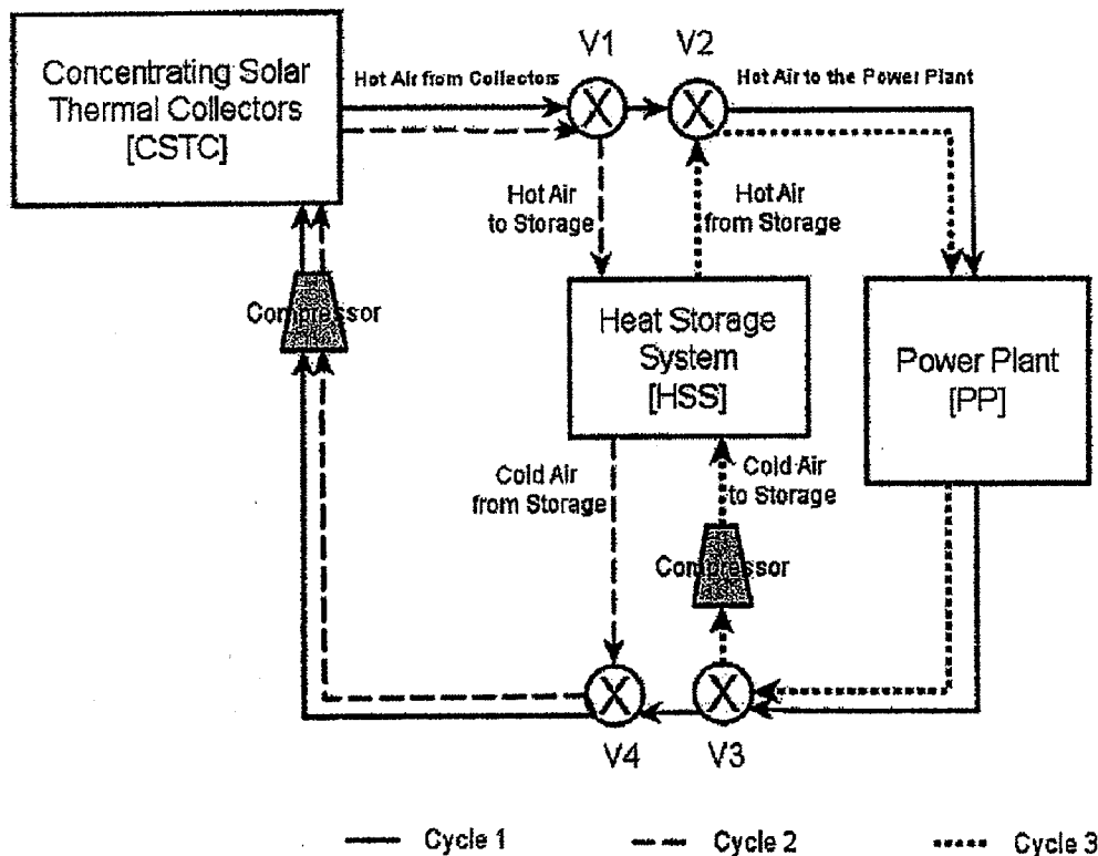
Concentrated Solar Energy with Heat Storage Capability
