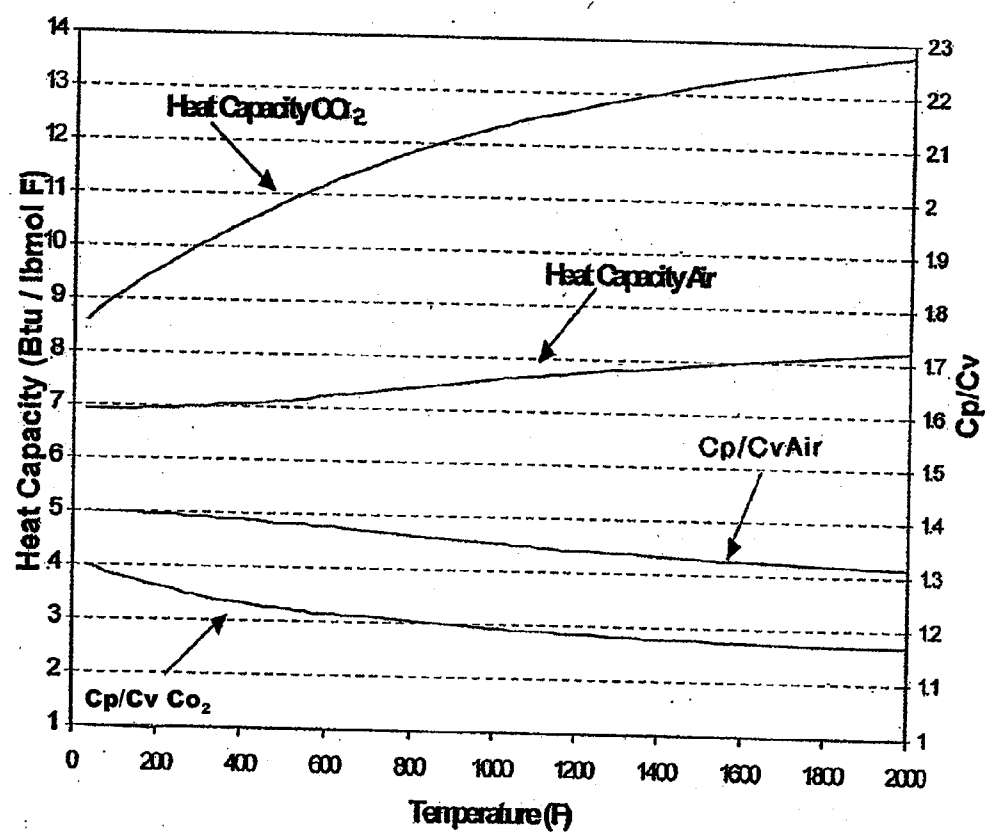
Figure 2. Heat Capacity and c_p/c_v Ratio for Air and CO_2
