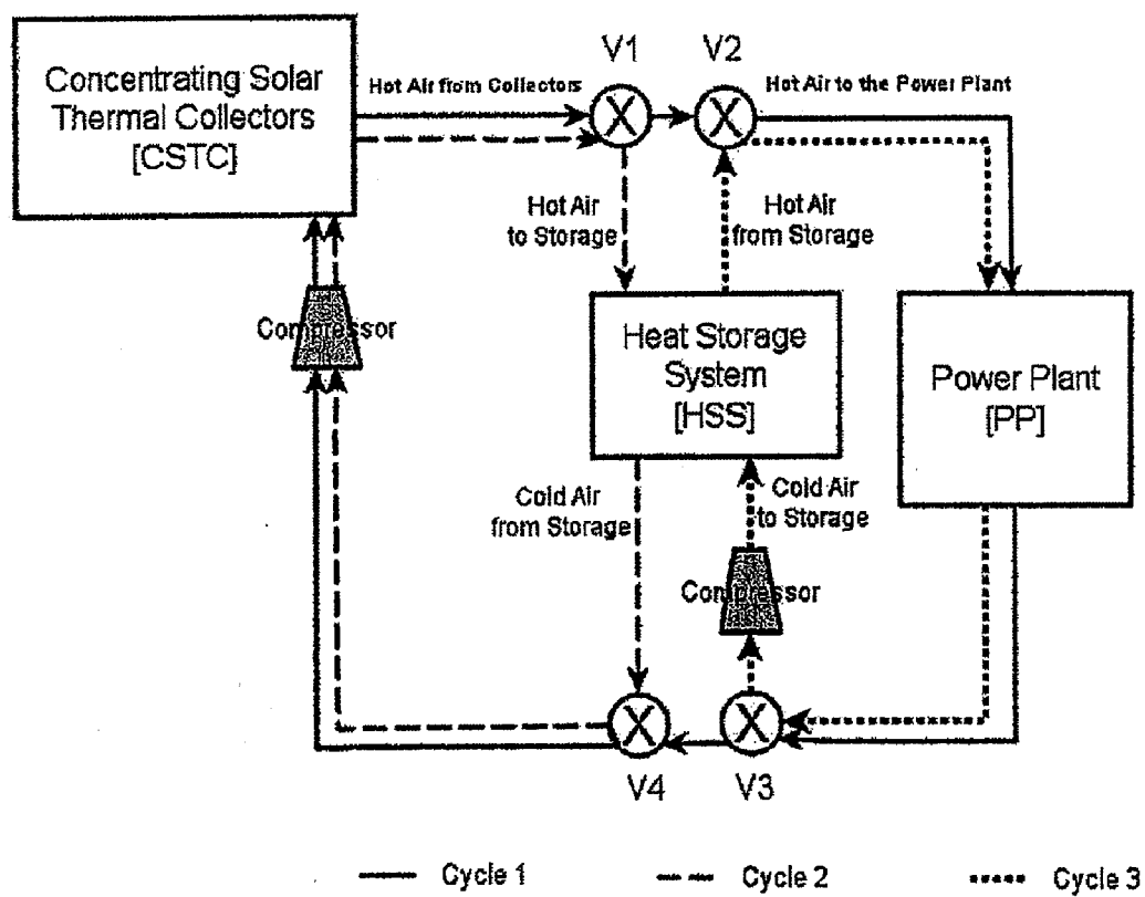
Figure 1: Concentrated Solar Energy with Heat Storage Capability
