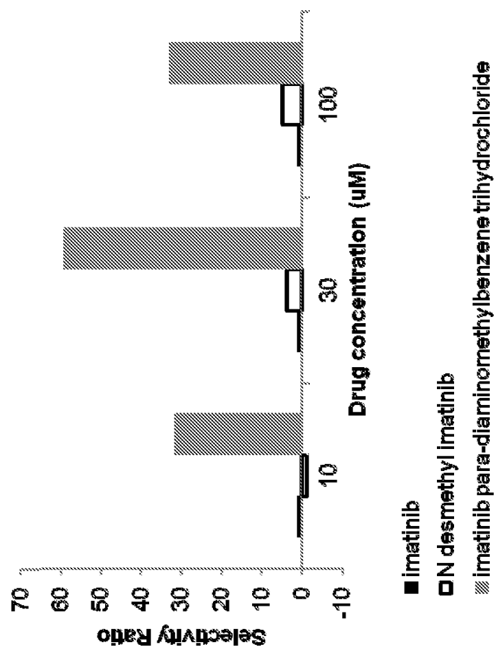
FIG. 9 Compound Selectivity
