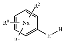
(Chemical formula 9)
