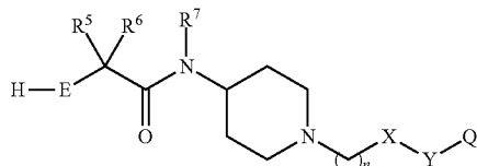
(Chemical formula 6)
