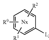
(Chemical formula 5)
