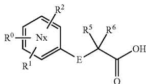
(Chemical formula 3)
