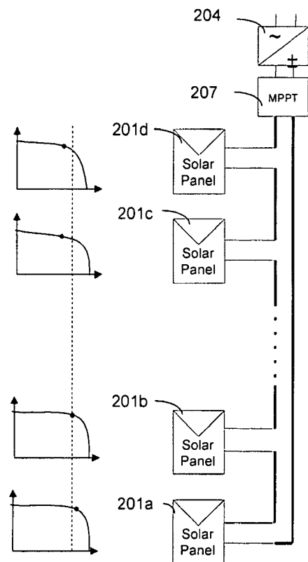
Figure 2 – Prior Art
