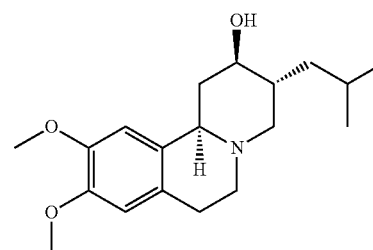
(+)-alpha-dihydrotetraabenazine
