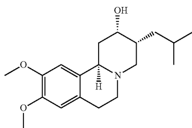
(+) -beta-dihydrotetrabenazine
