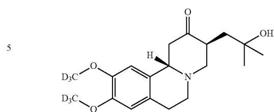
(3S, 11bS)-enantiomer
