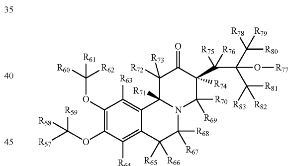
(3S, 11bS)-enantiomer
