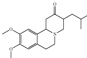
Tetrabenazine
