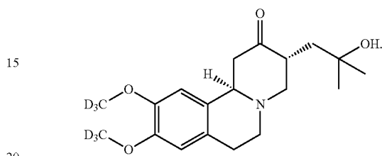
(3R, 11bR)-enantiomer
