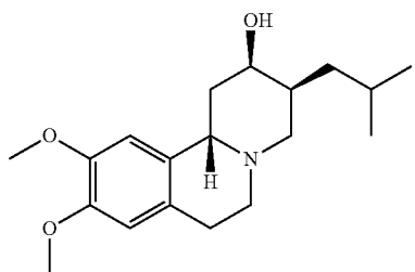
(-) -beta-dihydrotetrabenazine
