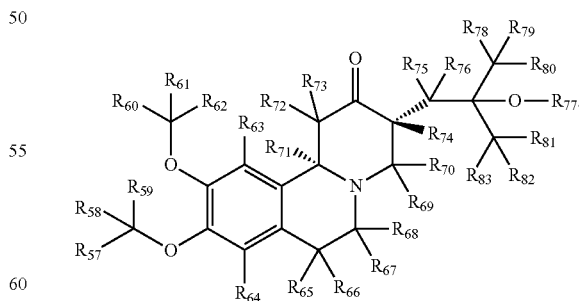
(3R, 11bR)-enantiomer
