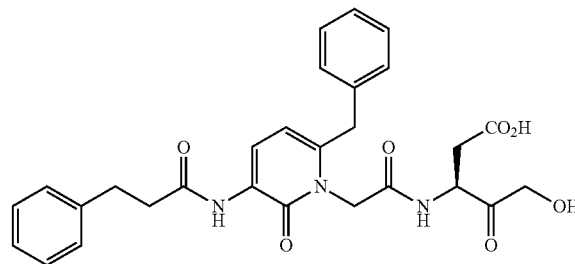
N-2-(6-Benzyl-1,2-dihydro-2-oxo-3-(3-phenylpropionyl)amino-1-pyridyl)acetyl-3(S)-amino-5-hydroxy-4-oxo-pentanoic acid (88)
