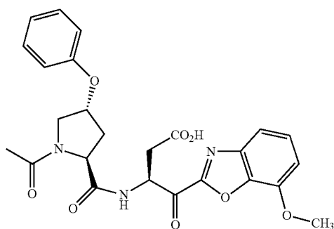
N-Acetyl-(4-(R)-phenoxy)prolinyl-3(S)-amino-4-(7-methoxybenzoxazol-2-yl)-4-oxo-butanoic acid (87)
