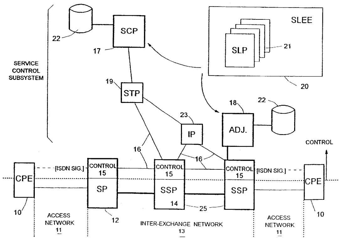
FIG. 2 (PRIOR ART)
