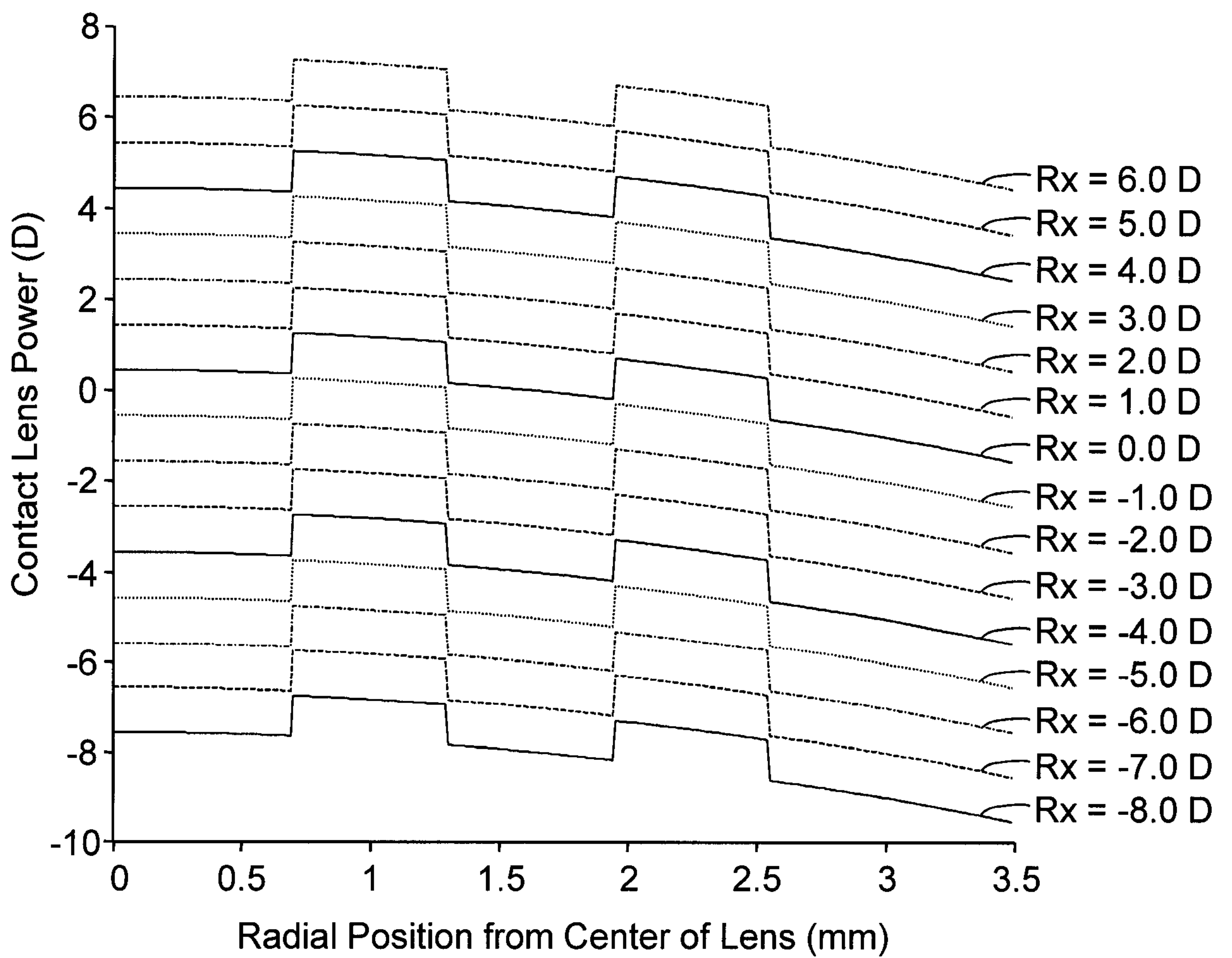
Contact Lens Power Profile for Select SKUs
