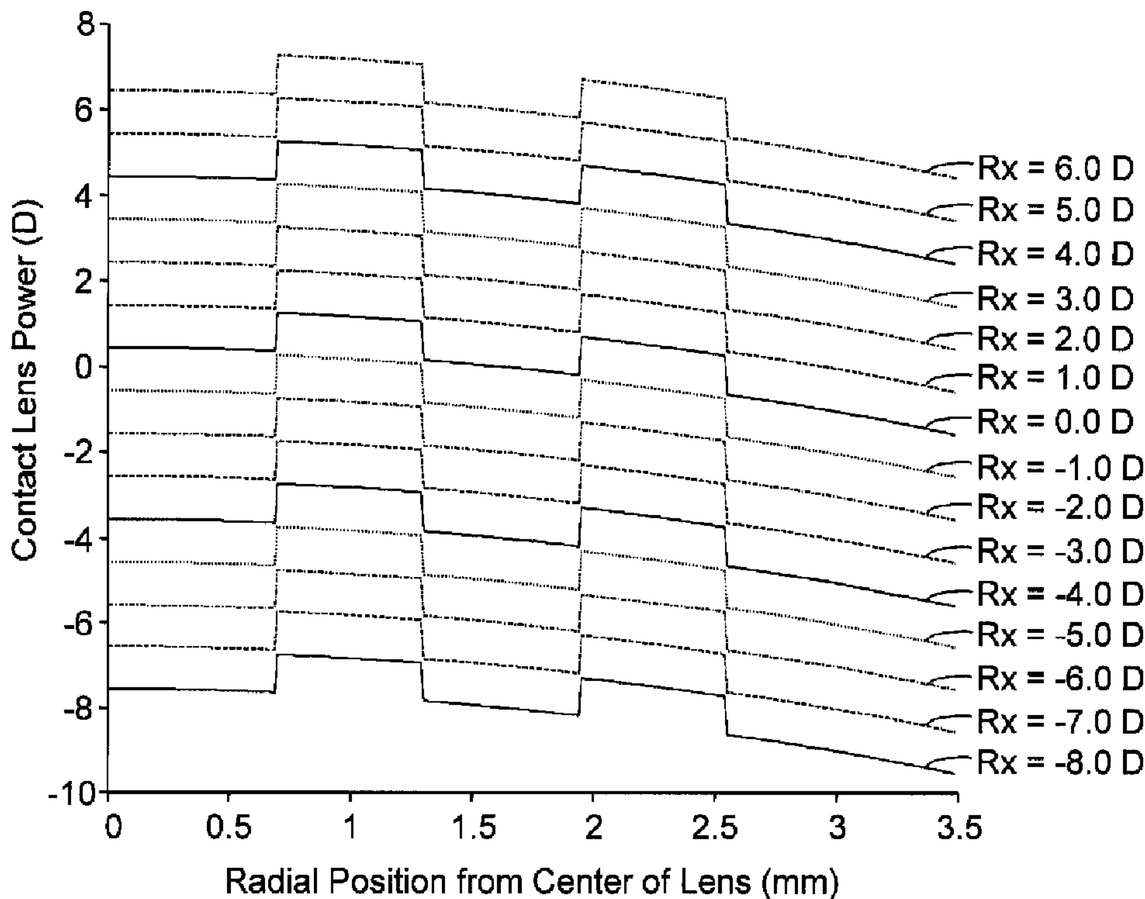
Contact Lens Power Profile for Select SKUs
