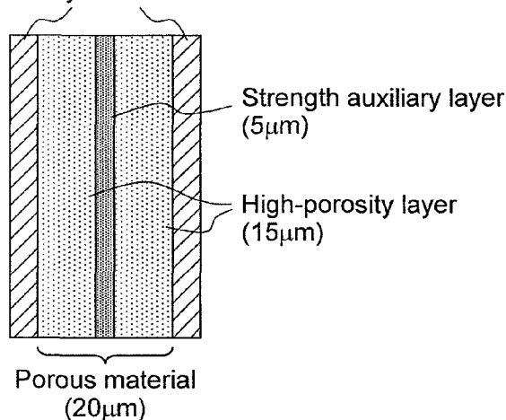
Electrolyte membrane
