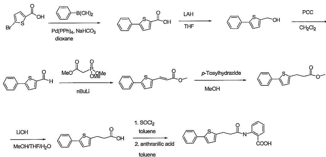
5 Scheme 12
