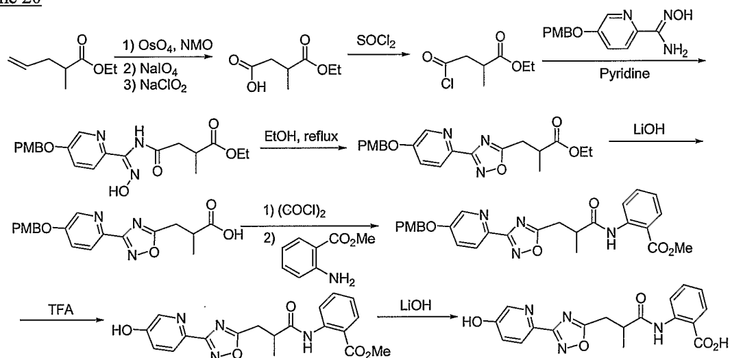
Scheme 20
